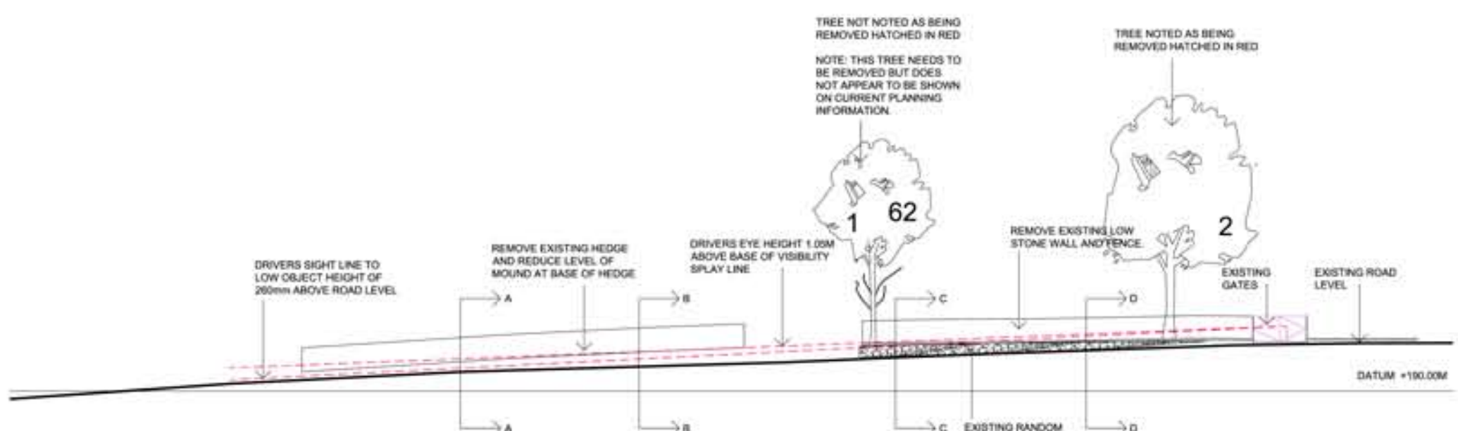
LONG SECTION THROUGH ROAD SHOWING ALTERATIONS TO FORM VISIBILITY SPLAY
